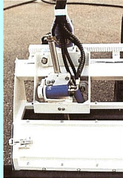
Carriage Lance support with 6 movements.
